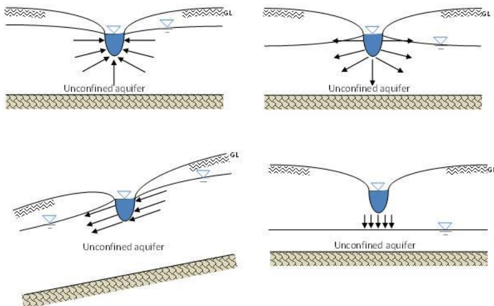
Fig. 1 Groundwater surface water interaction
