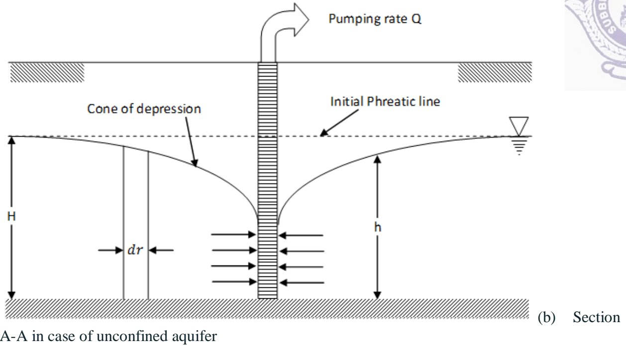
Fig. 15.4 An unconfined aquifer
