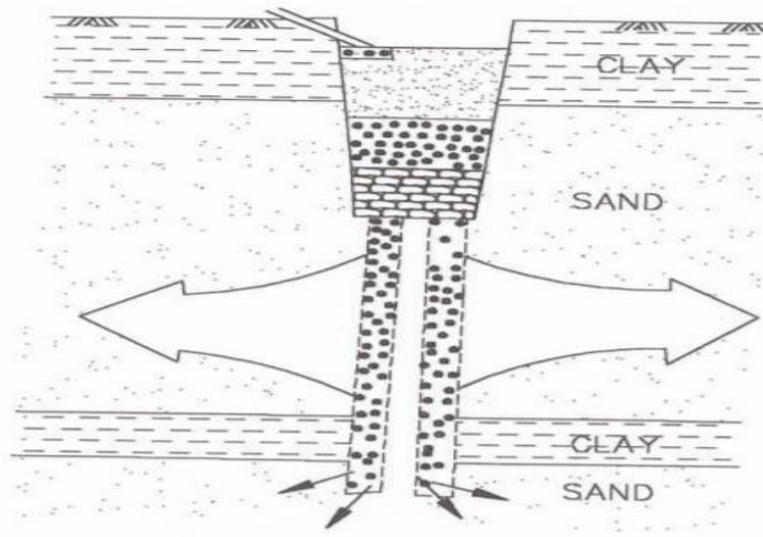
Figure 9.6 : Lateral Recharge Shaft
