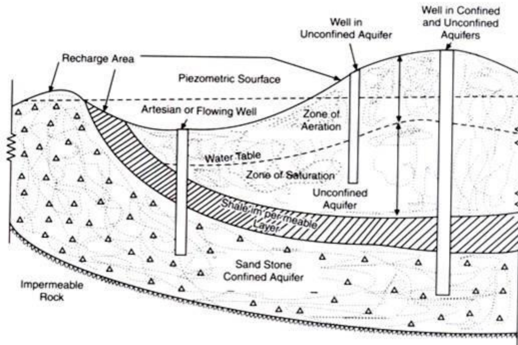
Fig. 16.4. Groundwater terminology model
