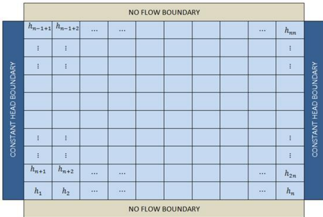
Fig. 7 Discretized aquifer
