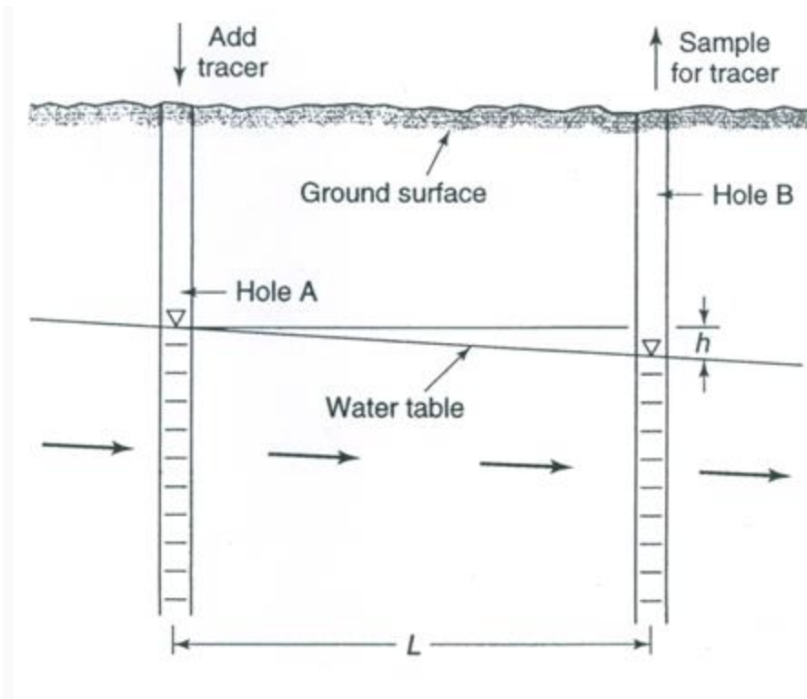
Fig. 12.3. Illustration of a tracer test in an unconfined aquifer for determining hydraulic conductivity. (Source: Mays, 2012)
