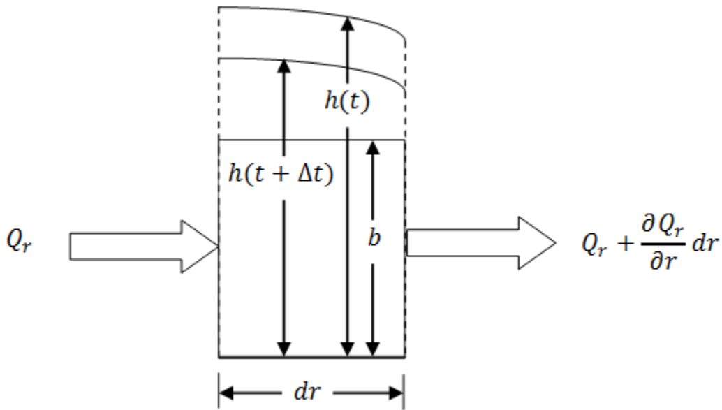
Fig. 15.3 Control volume in case of confined aquifer
