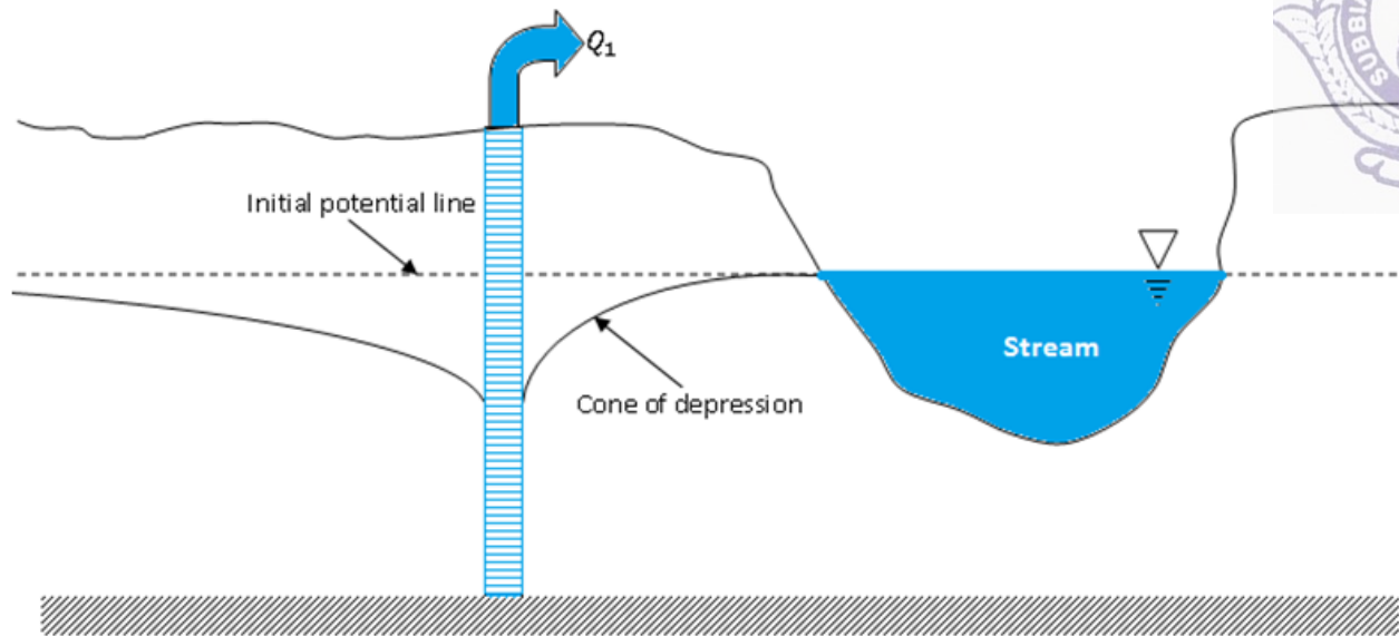
Fig. 21.3 Well near a stream
