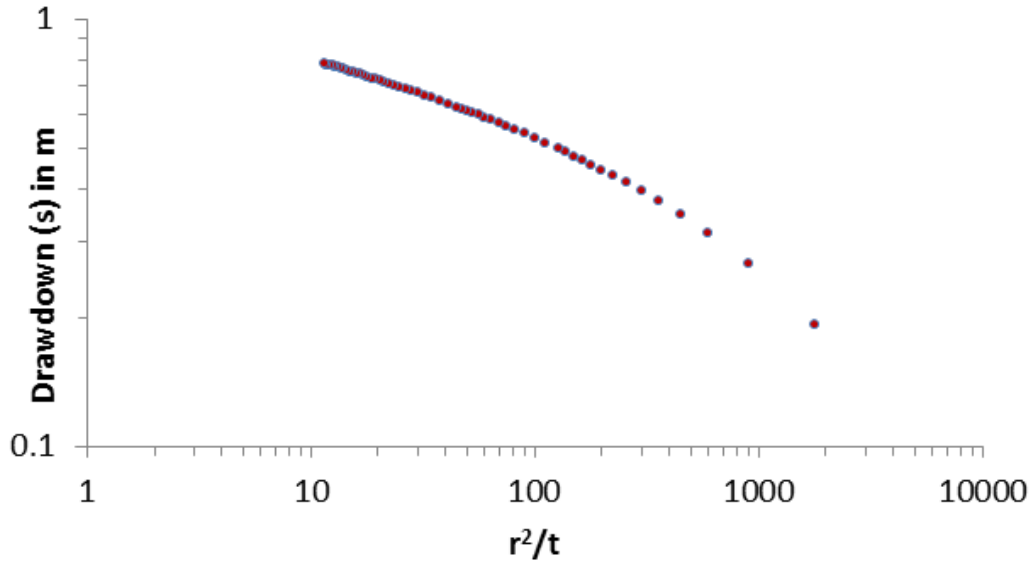
Fig 22.2 Relation between r^2/t and S
