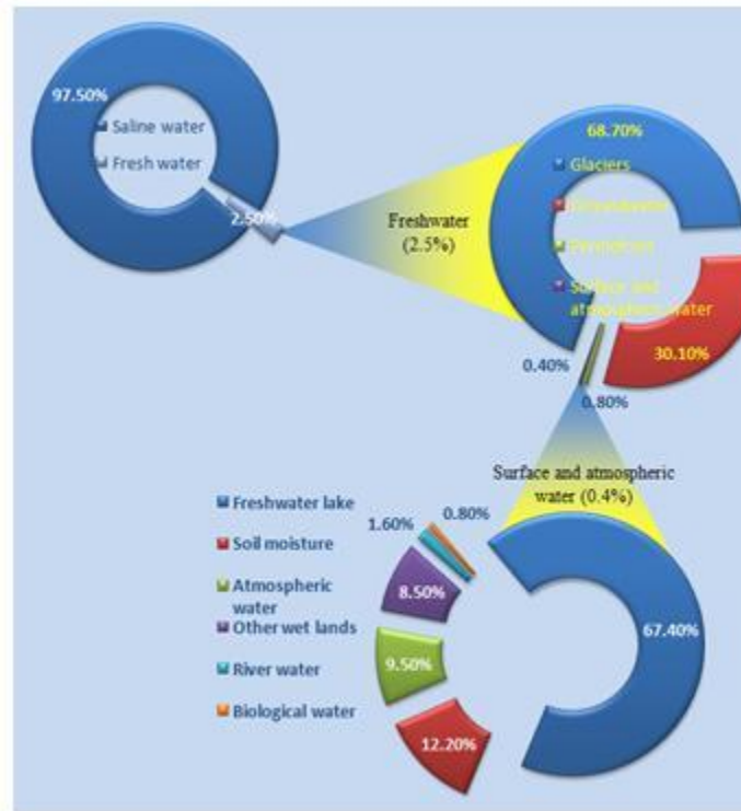
Fig. 2. 1 Global water distribution
