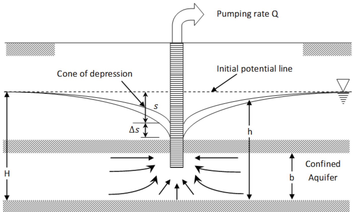
Fig. 20.1 Partially penetrated well
