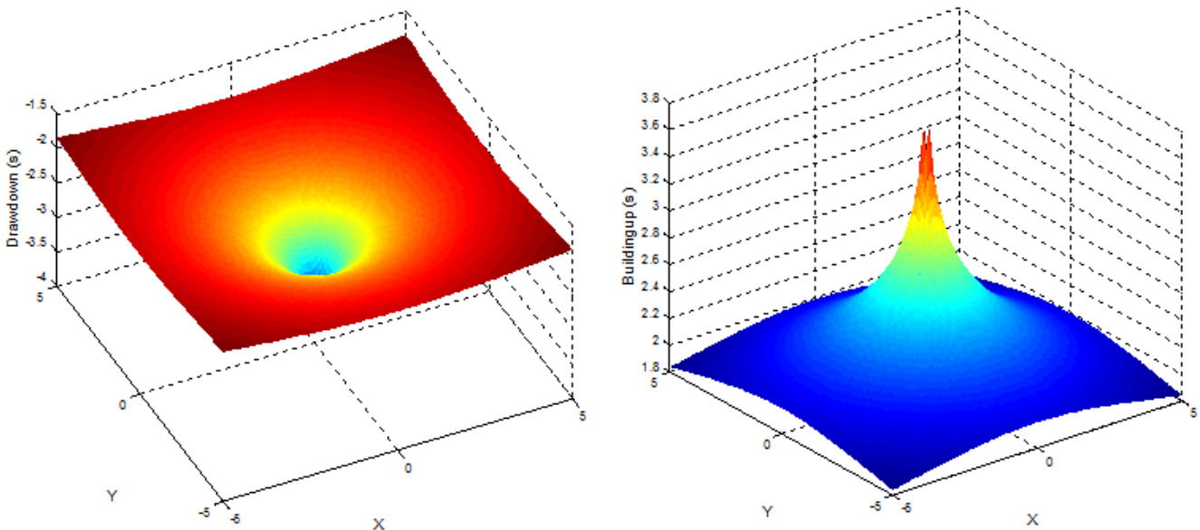
Fig. 15.1 (a) Cone of depression (b) Cone of impression
