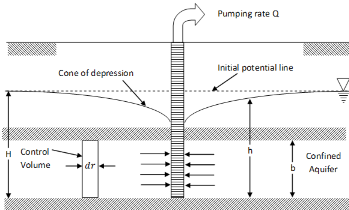
(b) Section A-A in case of confined aquifer
