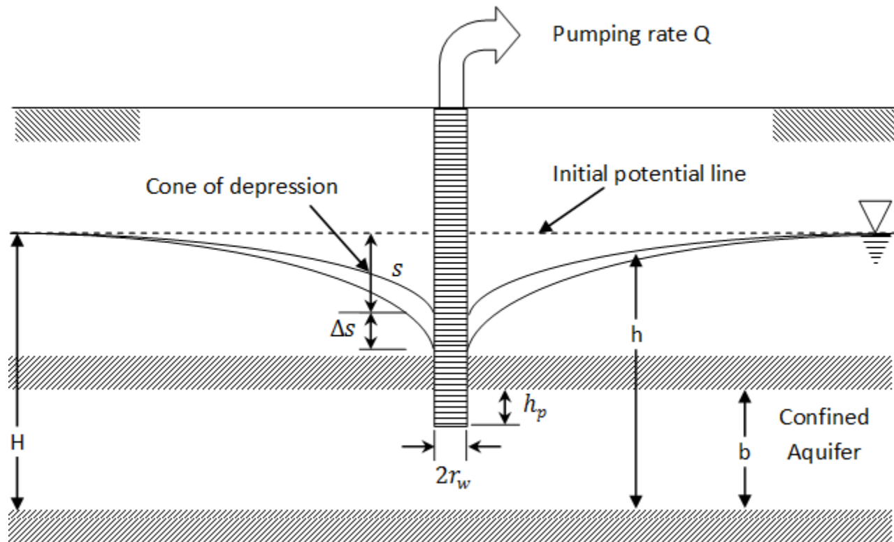
Fig. 20 .2 Partially penetrated well
