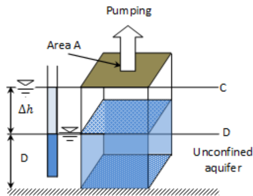
Fig.7.2 Sketch to explain aquifer storativity of unconfined aquifer
