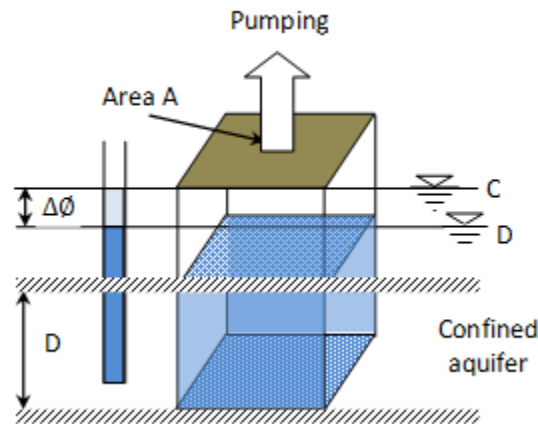
Fig. 7.1 Sketch to explain aquifer storativity of confined aquifer
