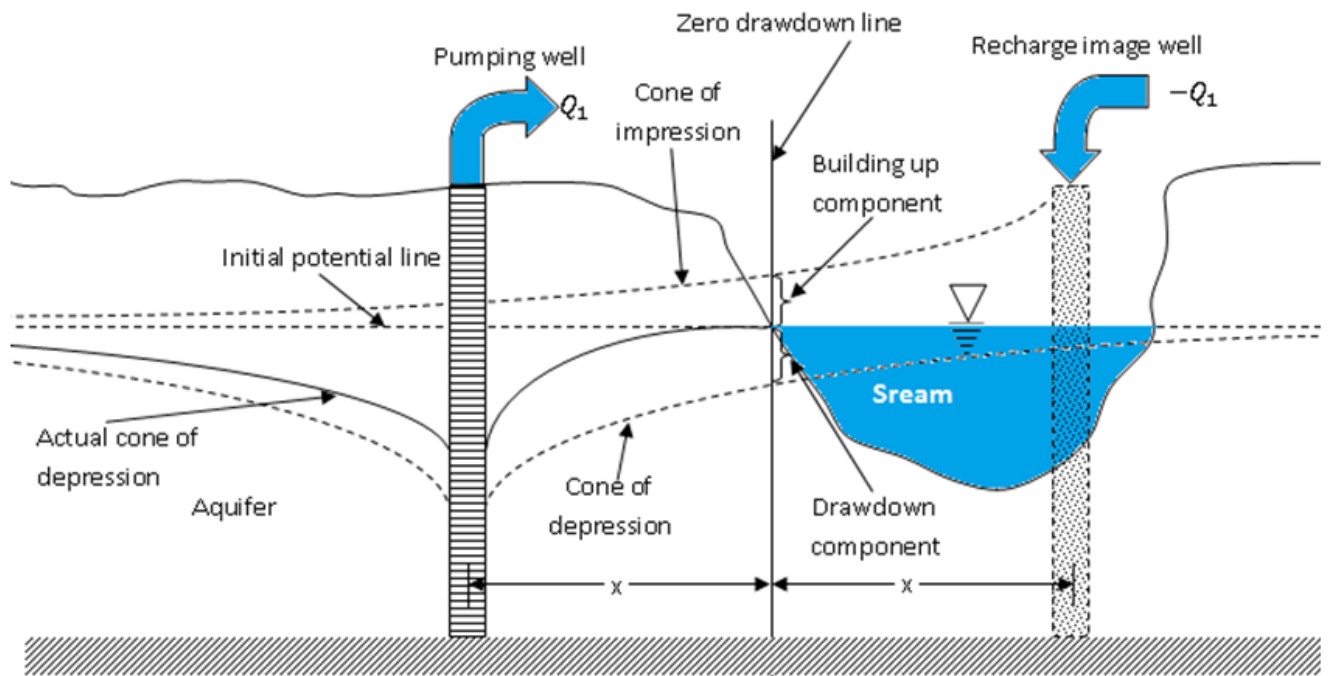
Fig. 21.4 Equivalent hydraulic system in a aquifer of infinite areal extend
