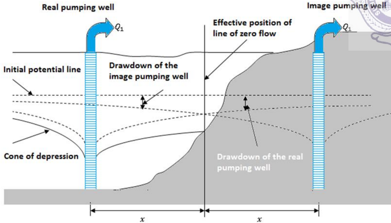
Fig. 21.7 Equivalent hydraulic system in a aquifer of infinite areal extend
