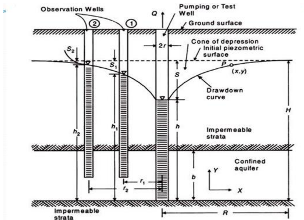
Fig Well penetrating confined aquifer
