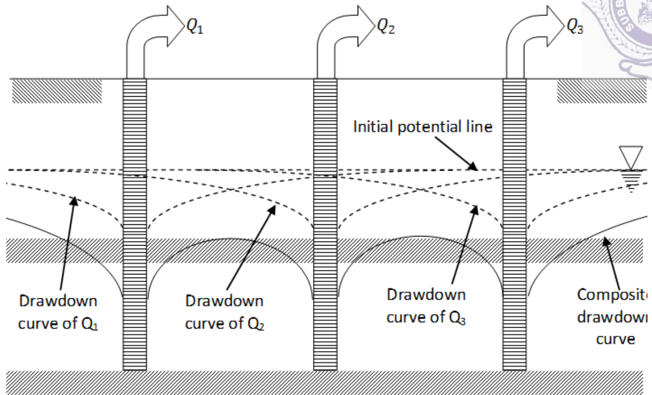
Fig. 21.1 Multiple well system
