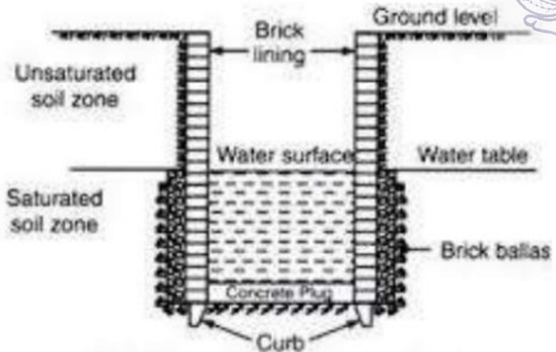
Fig. 17.1. Well with pervious lining
