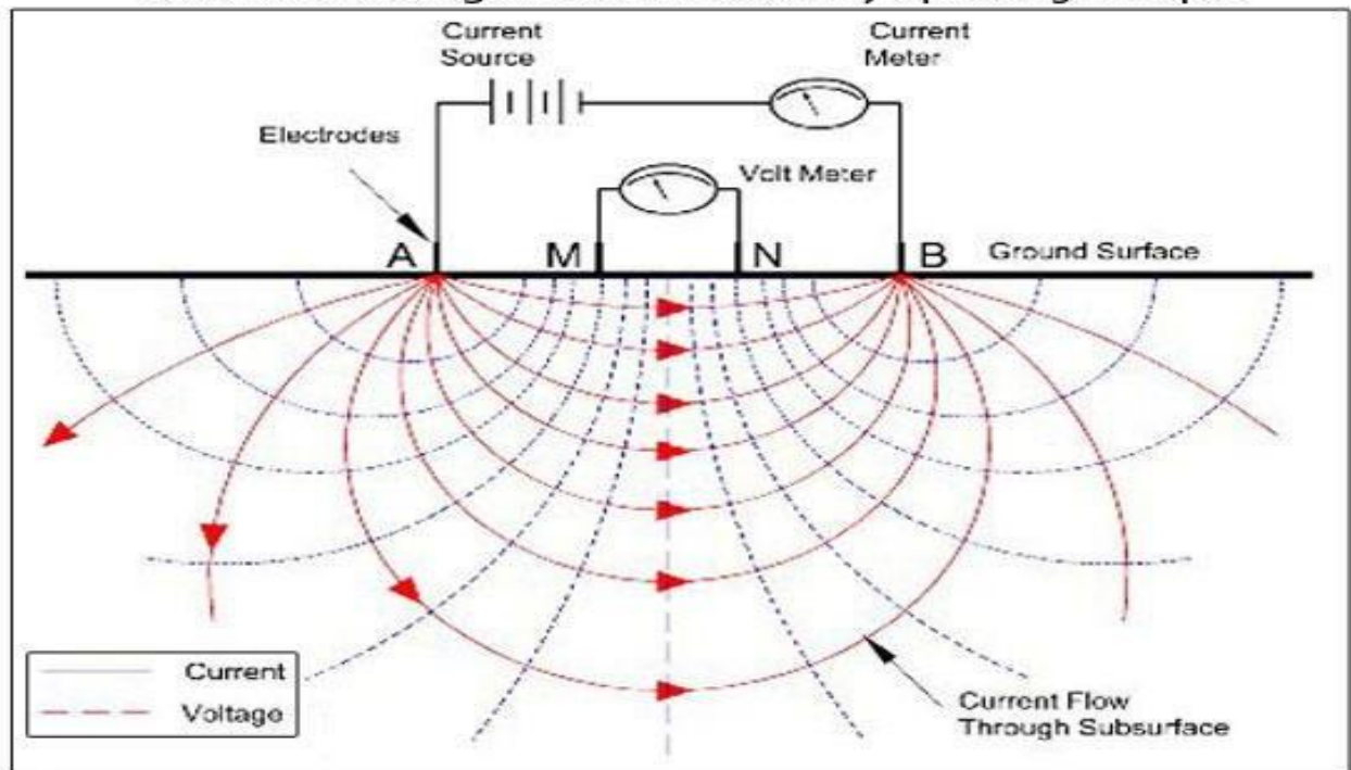
Schematic Drawing of Electrical Resistivity Operating Principles
