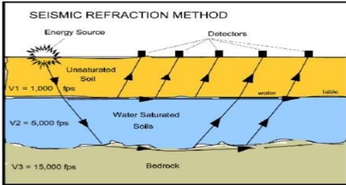
Fig 1 Seismic Refraction Method
