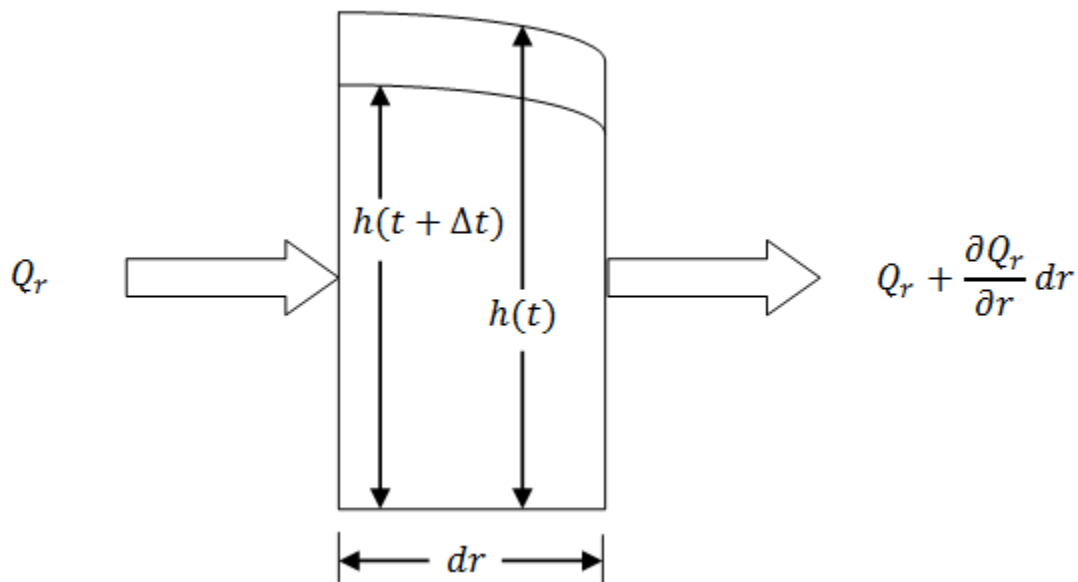
Fig. 15.5 Control volume
