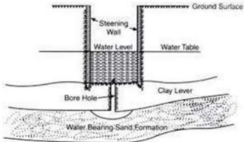
Fig. 17.2. Well with impervious lining
