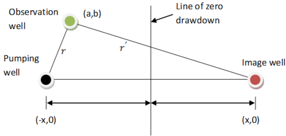
Fig. 21.5 Pumping well, Observation well and Image well
