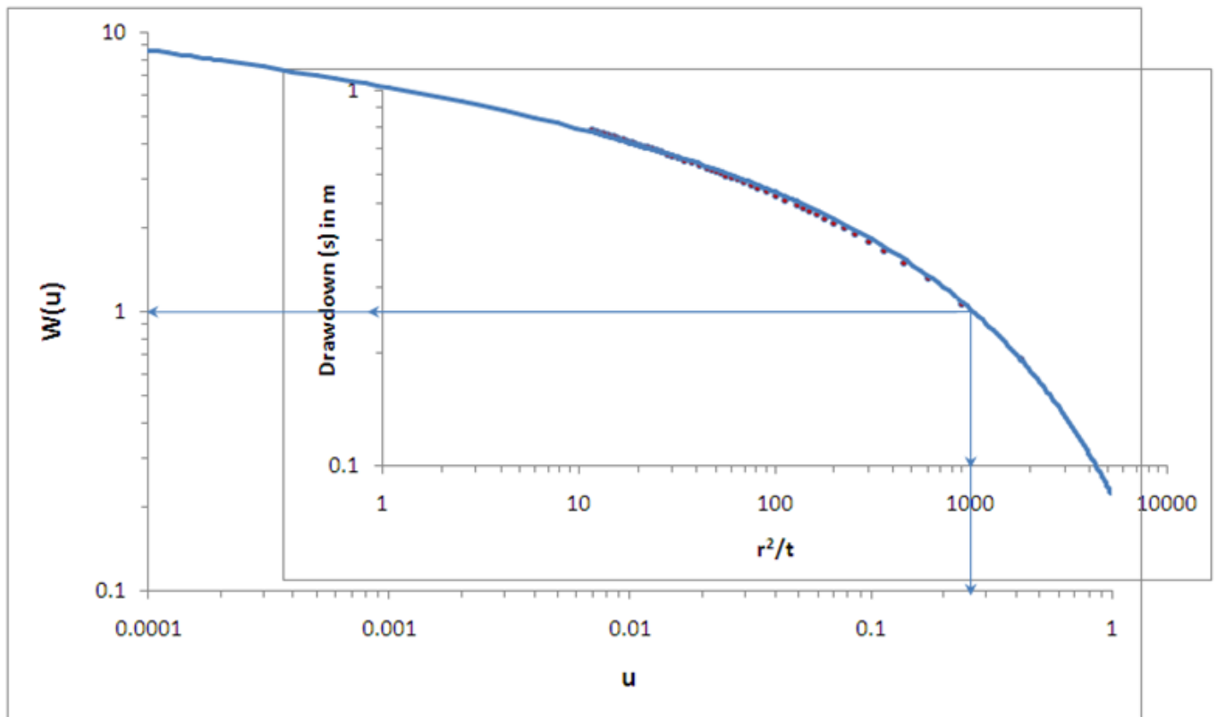
Fig 22.3 Superimposition of the relation between W(u) and u , and r^2/t and S
