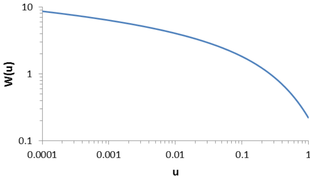
Fig.22.1 Relation between W(u) and u
