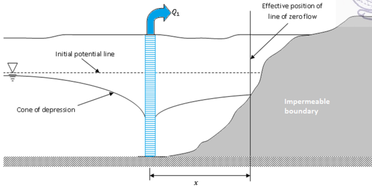
Fig. 21.6 Well near an impermeable boundary
