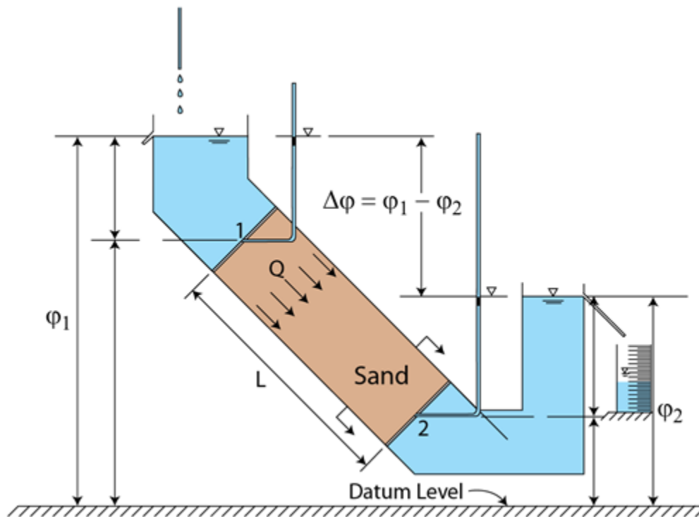
Fig. 3.2: Darcy's Experiments in inclined sand filter
