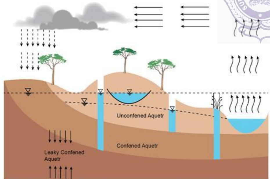
Fig.1.1 Hydro-geological cycle
