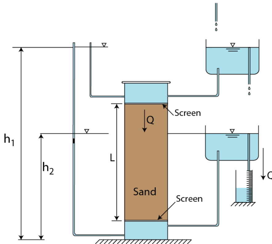
Fig. 3.1 Darcy's Experiment in vertical sand filter
