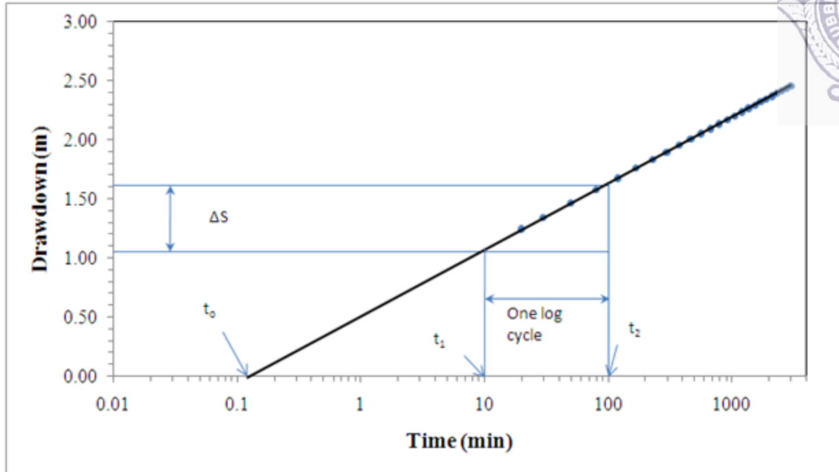
Fig 22.4 Observed time drawdown relation with time in log scale
