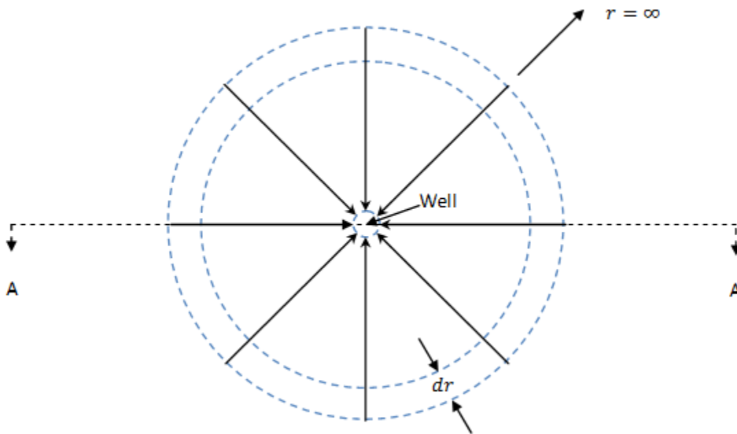
(a) Radial flow to a well
