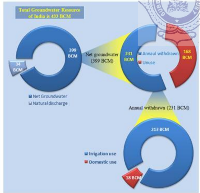
Fig. 2. 2 Groundwater resource of India
