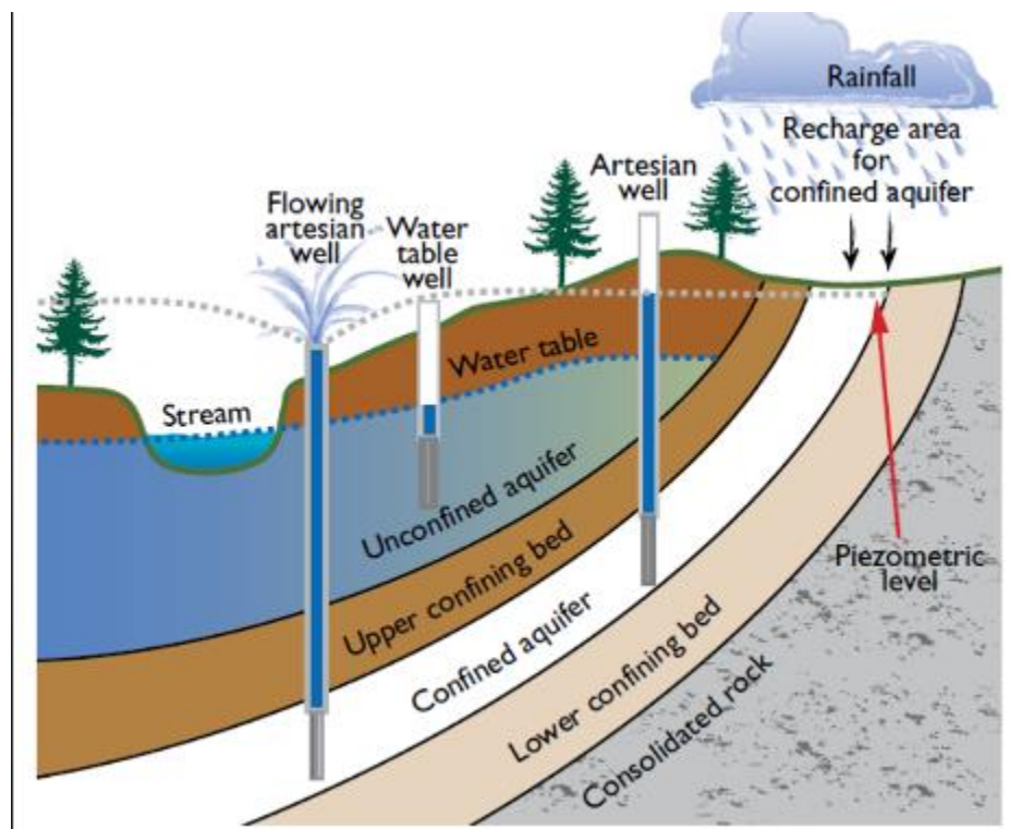
Confined and Unconfined aquifer
