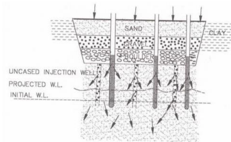
Figure 9.6 : Lateral Recharge Shaft
