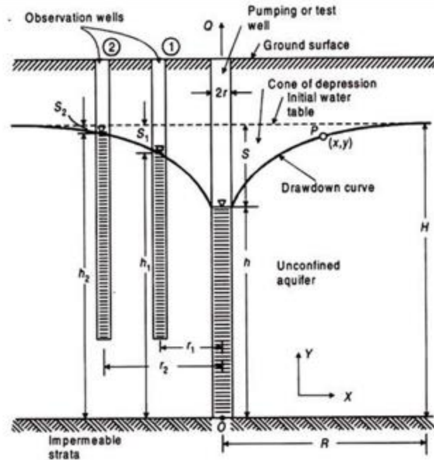
Fig Well penetrating an unconfined aquifer
