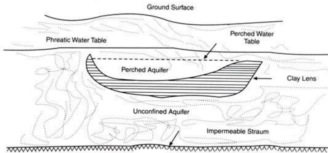
Fig. 16.3. Unconfined and perched aquifers
